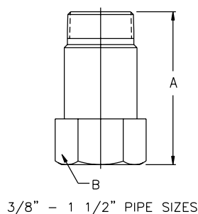
3/8" - 1 1/2" PIPE SIZES
