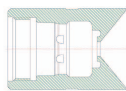
Carrier 10 (CI10) (shown) Carrier 12 (CI12) - without lugs
