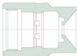
Carrier 1 (CI1) (shown) Carrier 11 (CI11) - without lugs
